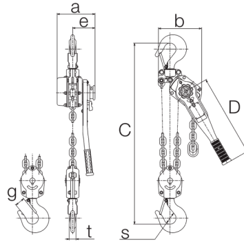
L5LB 6 Metric Tonne line drawing
