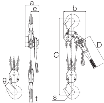
L5LB 9 Metric Tonne line drawing
