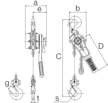
L5LB ¾ - 3 Metric Tonne line drawing
