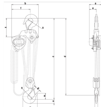
M3CB 7½ and 15 Metric tonne line drawing
