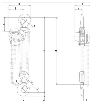
M3CB 3 - 5 Metric tonne line drawing
