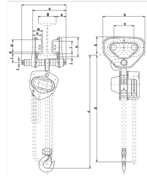
M3CB with TSP line drawing
