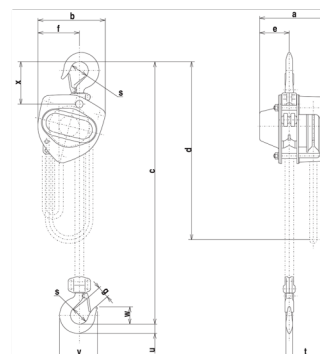
M3CB 1/2 - 2 1/2 Metric tonne line drawing
