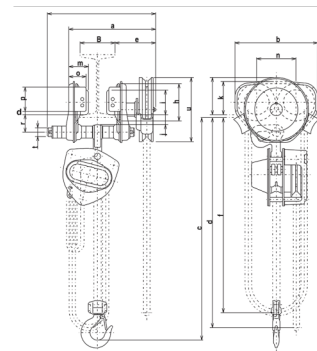
M3CB Geared Trolley Mount
