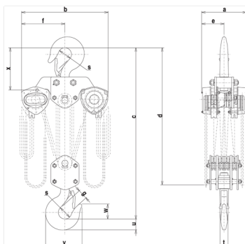
M3CB 20 and 50 Metric tonne line drawing
